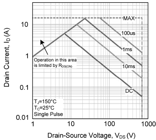
5. Maximum Safe Operating Area
