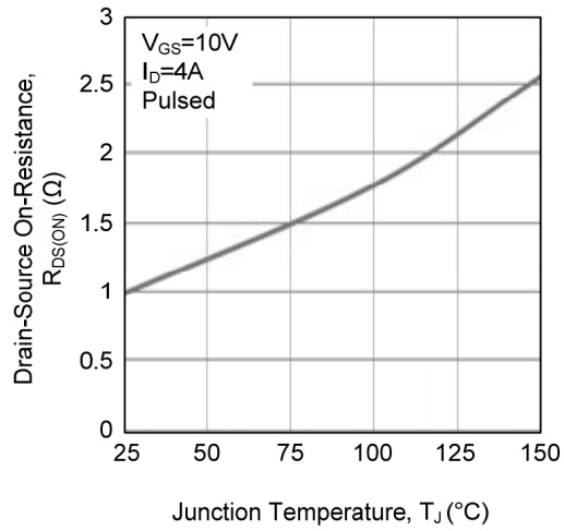
2. Drain-Source On-Resistance vs. Junction Temperature
